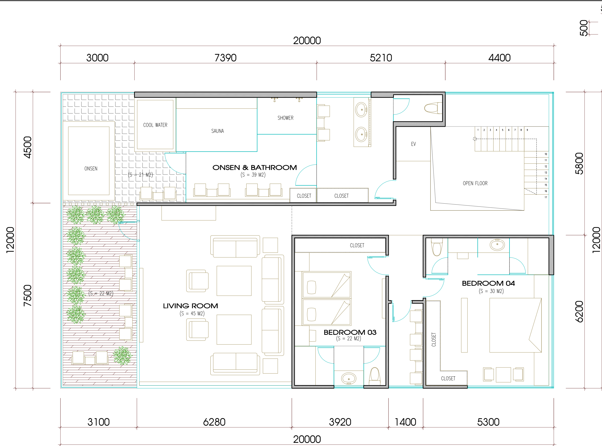
2ND FLOOR PLAN S = 240 M 2
